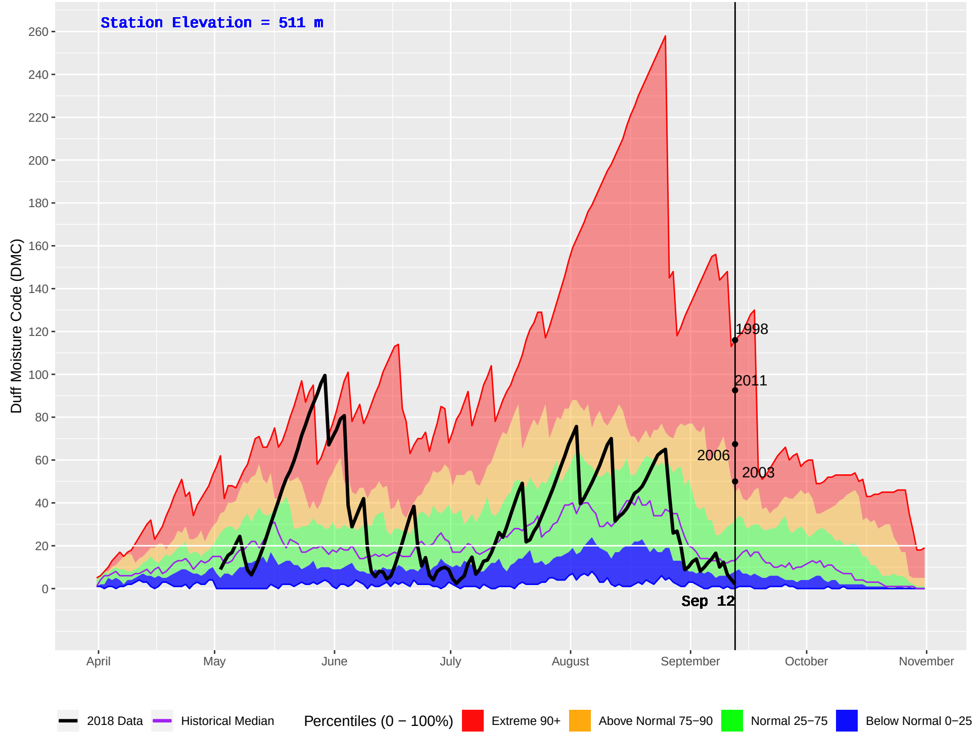
SEYMOUR ARM (344) : Historical (1981–2016) and Current (2018) Daily Duff Moisture Code (DMC)
