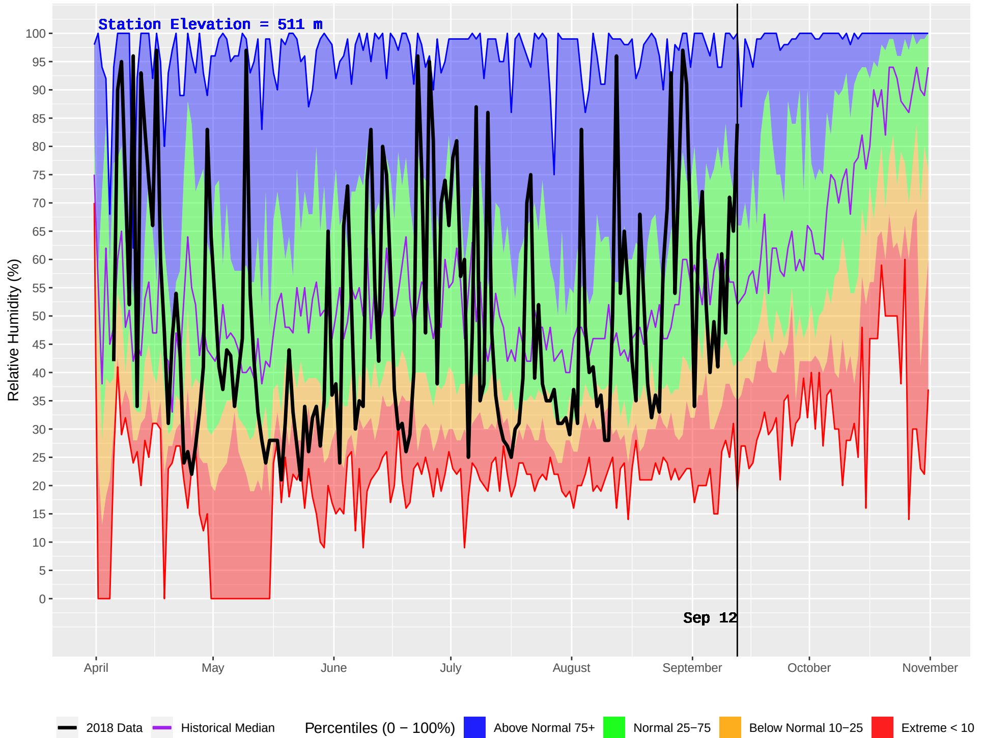
SEYMOUR ARM (344) : Historical (1981–2016) and Current (2018) Daily Relative Humidity
