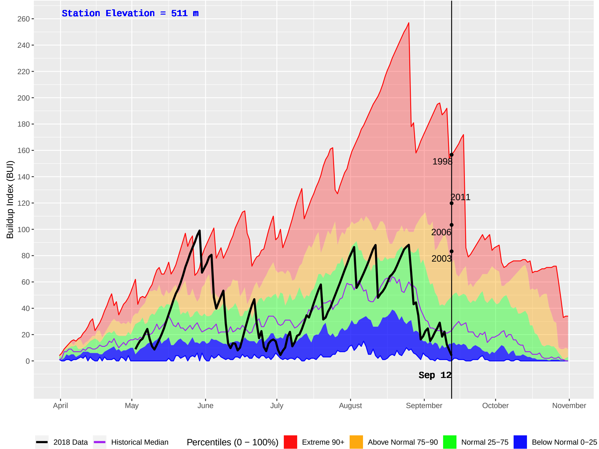
SEYMOUR ARM (344) : Historical (1981–2016) and Current (2018) Daily Buildup Index (BUI)
