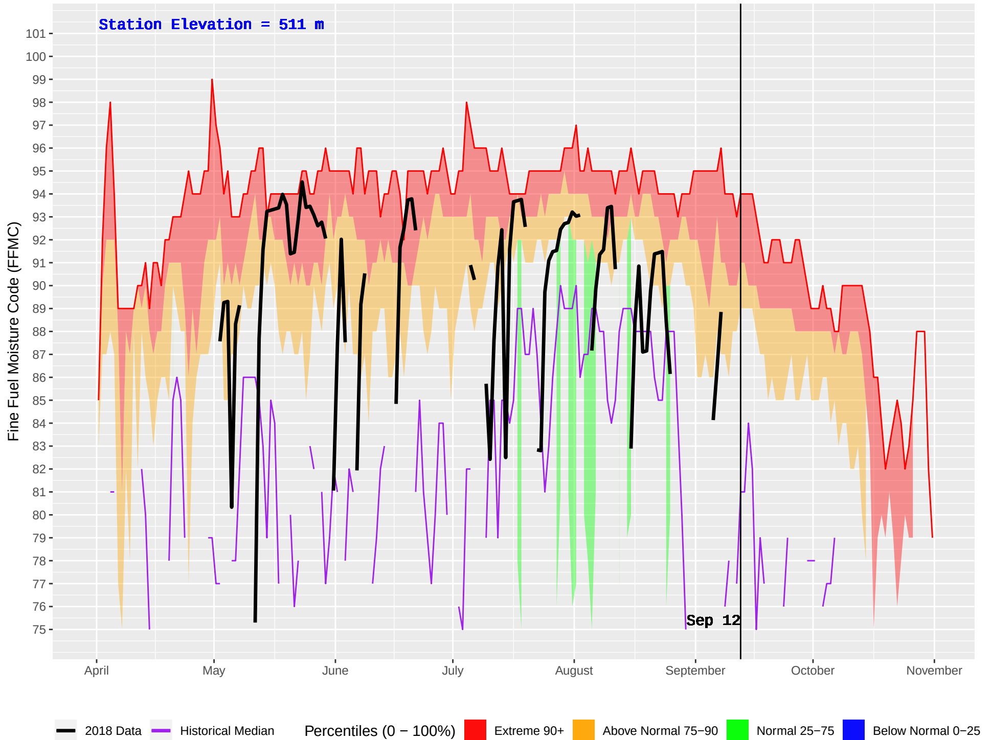
SEYMOUR ARM (344) : Historical (1981–2016) and Current (2018) Daily Fine Fuel Moisture Code (FFMC)
